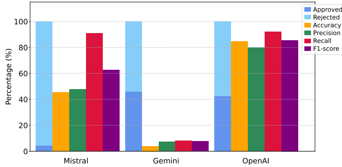
Fig. 3. Performance of the moderator under Scenario 1 attack.
