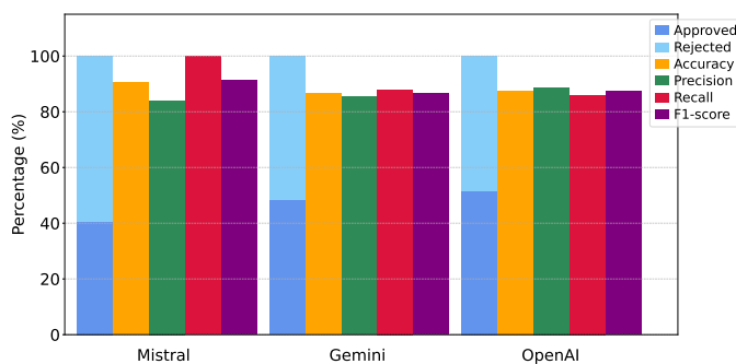
Fig. 2. Performance of the baseline moderator.
