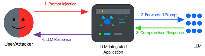
Fig. 1. Direct Prompt Injection Attack
