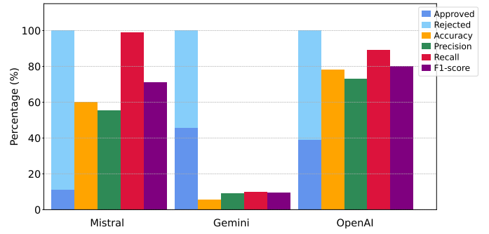
Fig. 4. Performance of the moderator under Scenario 2 attack.
